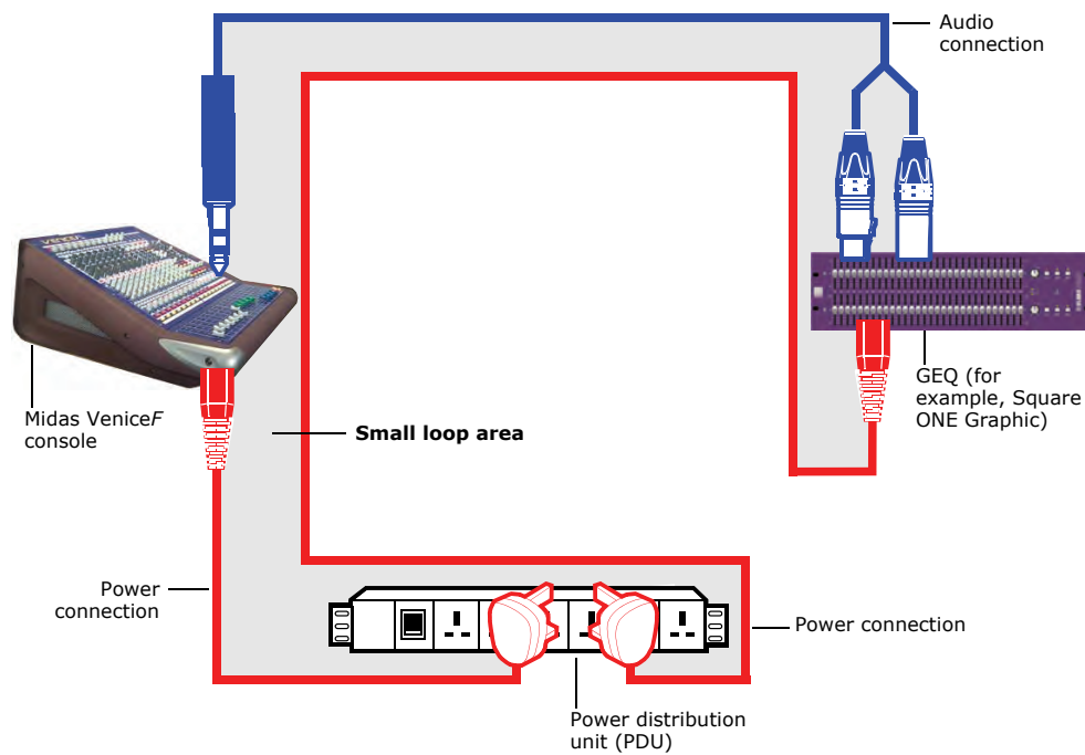
Loop area diagram showing a small loop area
