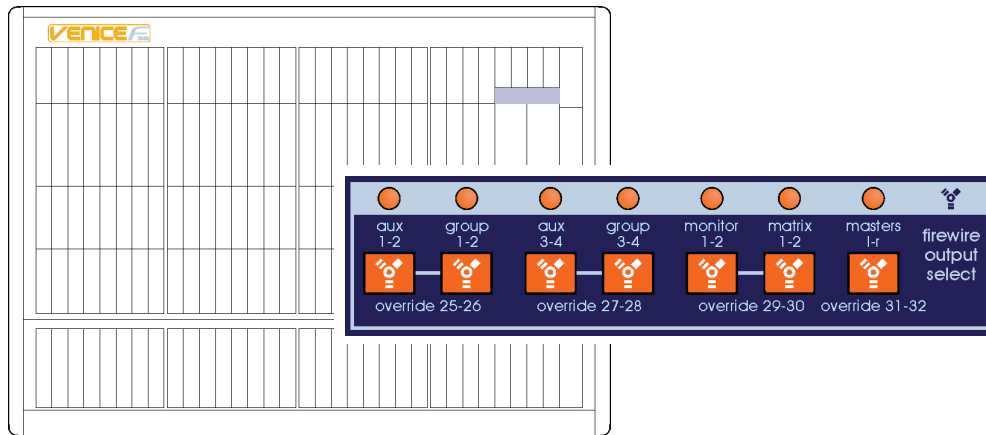
firewire output select section on the control surface
