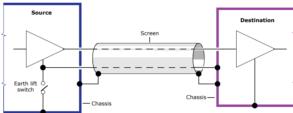
Ground lift connection on source
