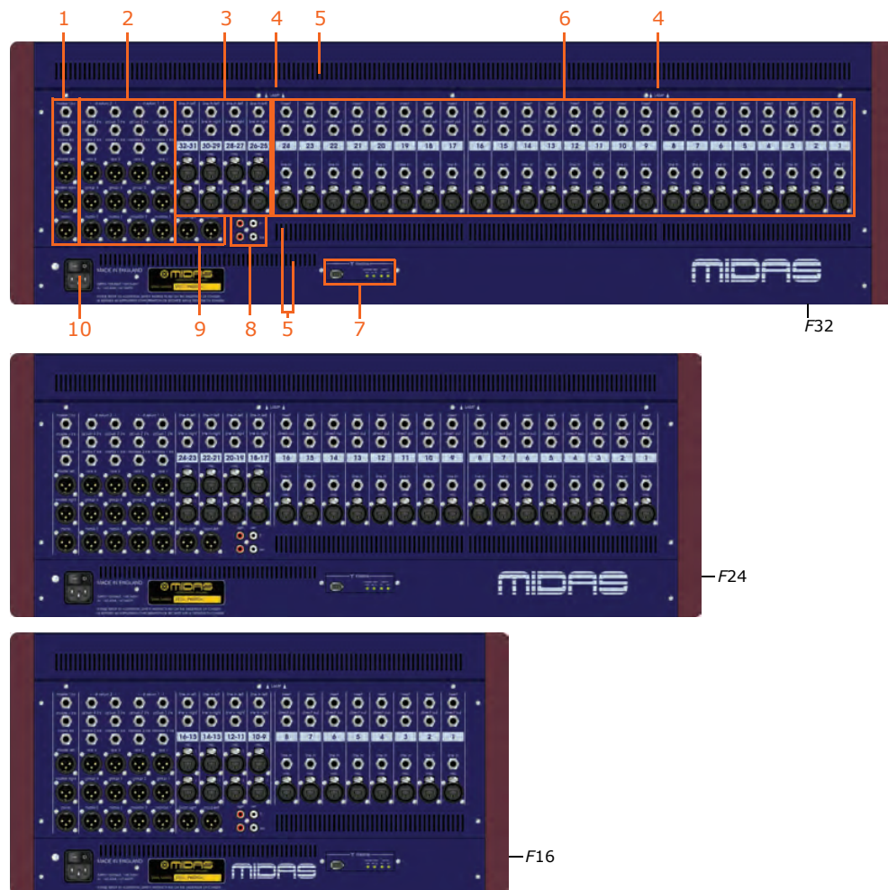
Rear panels of the VeniceF consoles showing the main areas
