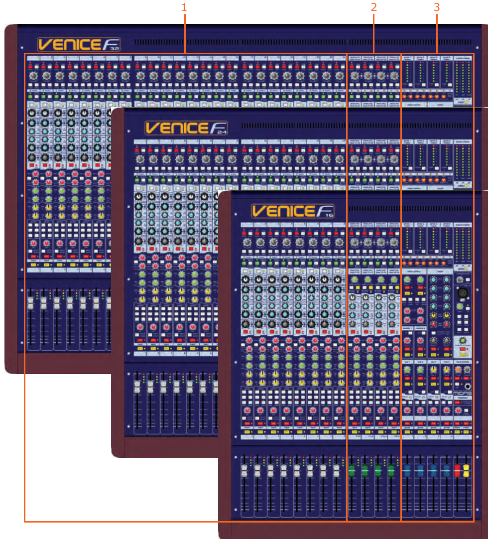
Control surfaces of the VeniceF consoles showing the three mains areas
