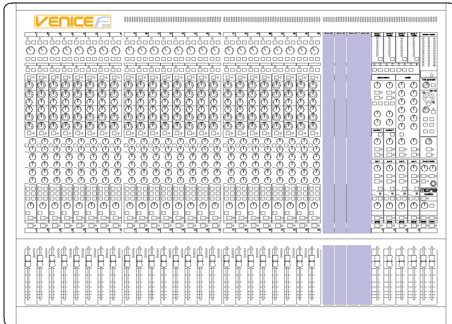
Dual stereo input channels on the control surface
