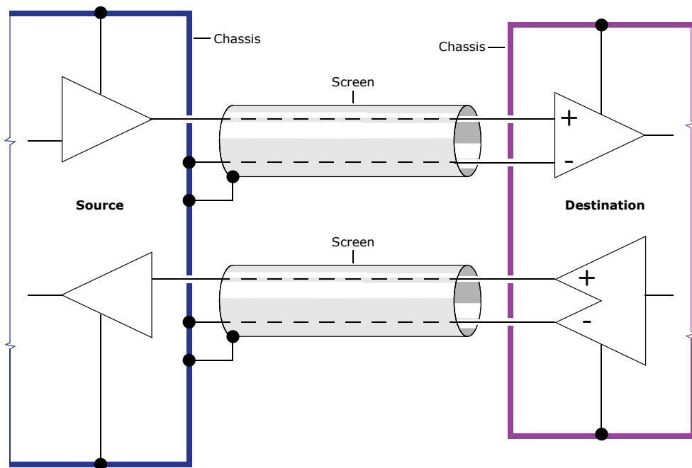
Ground referenced insert wiring diagram. For a typical example of how to wire a ground referenced insert, see Figure 1 on page 14; the example above shows the screen connection at the other end because it is more practical, as it reduces the wiring complexity within the 1/4" TRS Jack connector.
