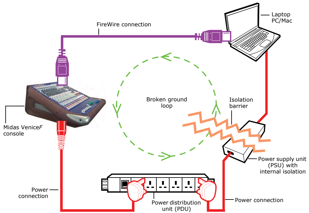
Isolated FireWire computer system. Note how the isolation barrier breaks the ground loop.
