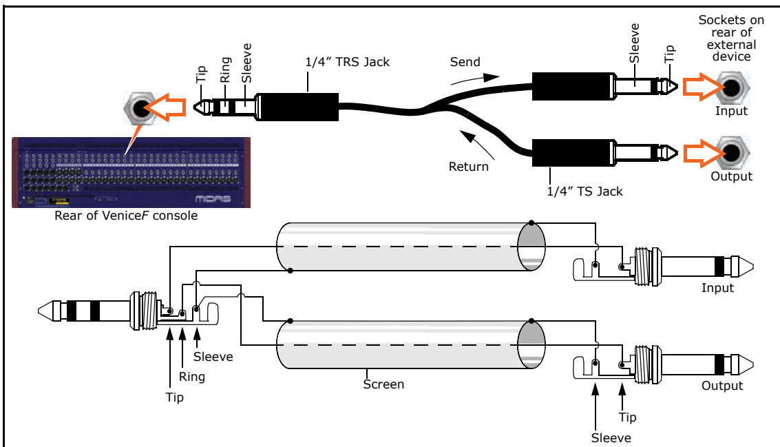
Figure 2: Connecting to unbalanced equipment
