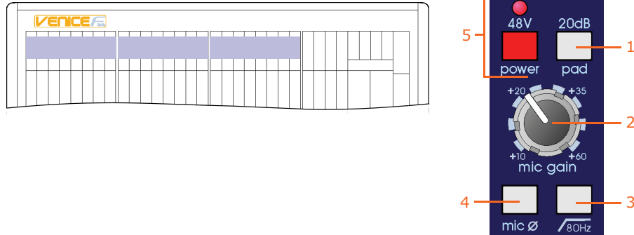
Mic gain section of the mono input channels
