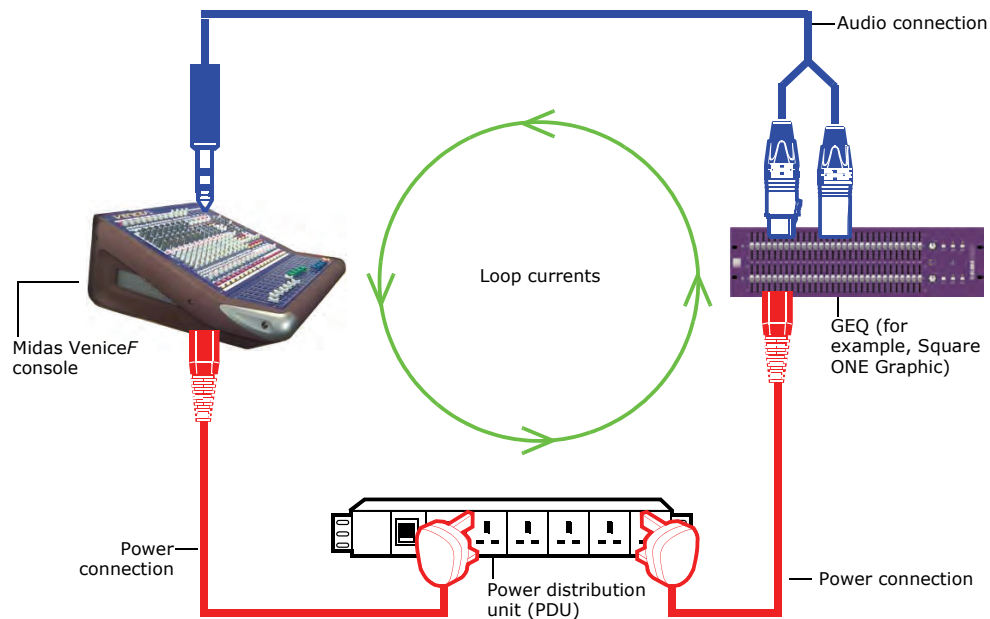
Ground loop
