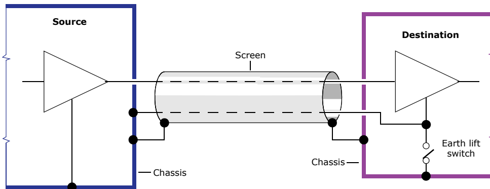
Ground lift connection on destination
