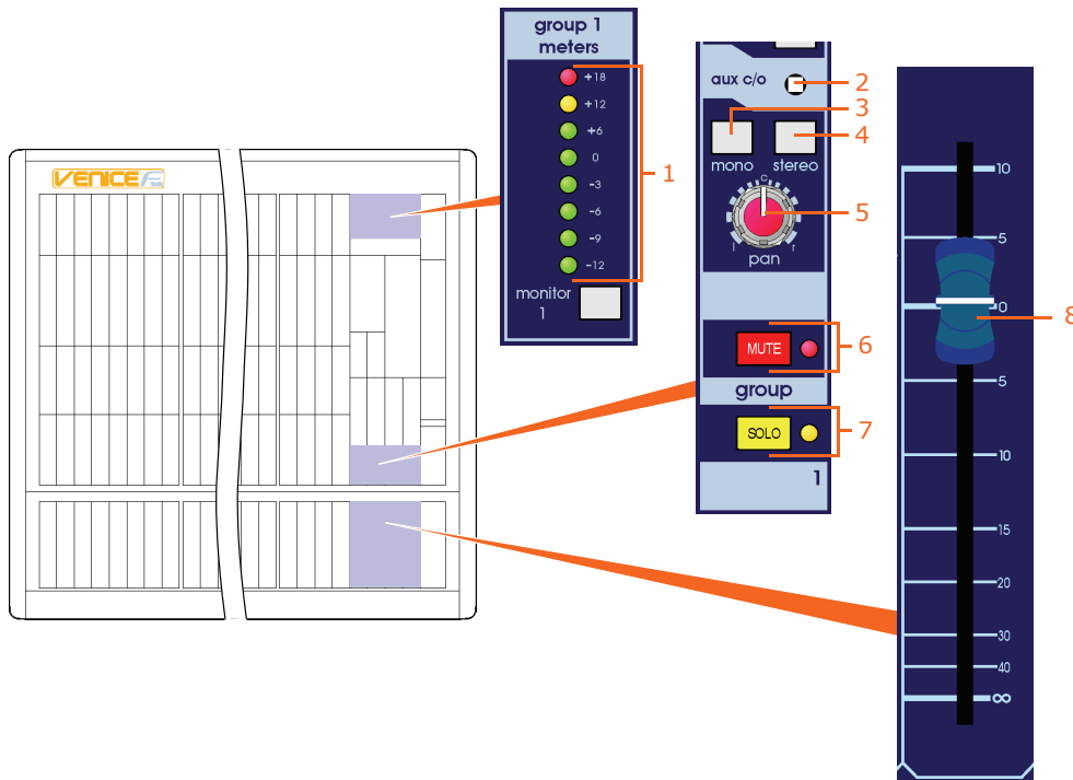
Group output sections on the control surface
