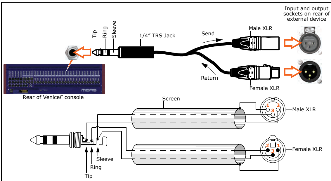
Figure 1: Connecting to balanced equipment
