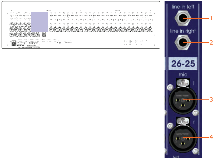
Dual stereo input channel connectors
