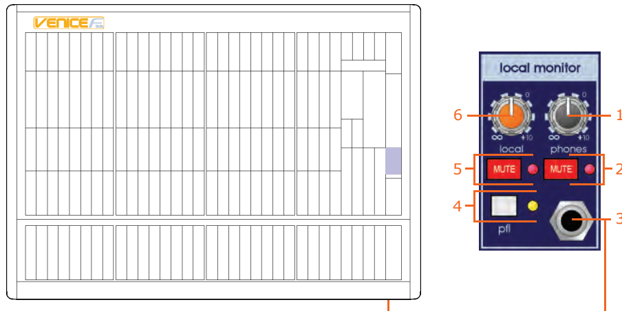
Local monitor section on the control surface and the position of the addition headphones socket on the front panel of the console
