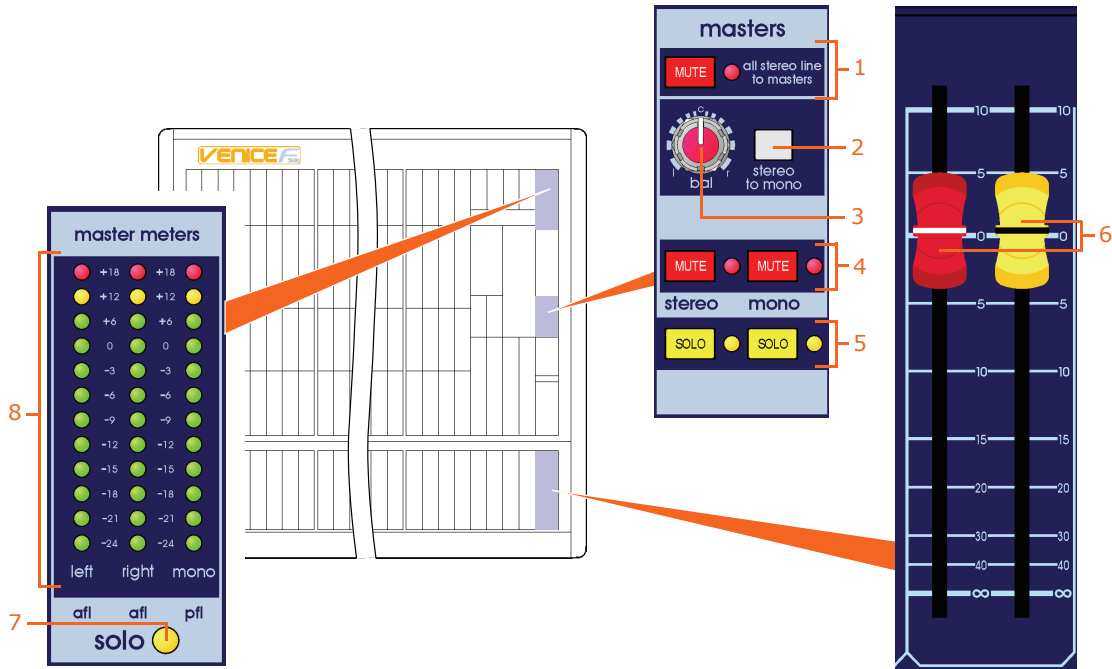
Master outputs sections on the control surface
