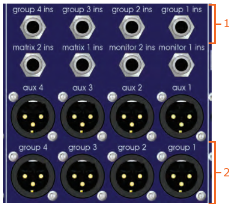
Group connectors on rear panel
