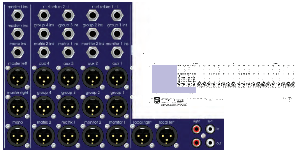
Output connections on rear panel
