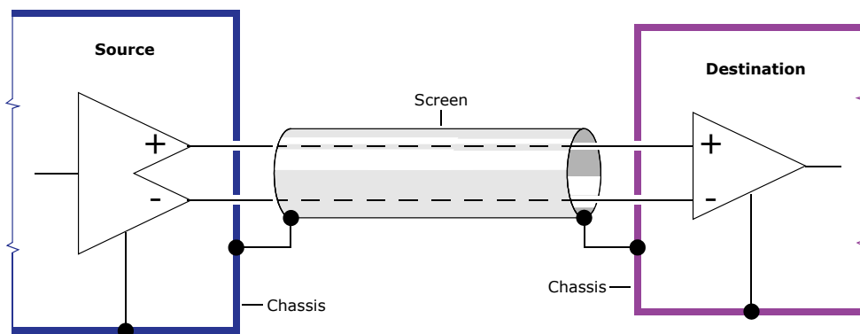
Balanced connection diagram
