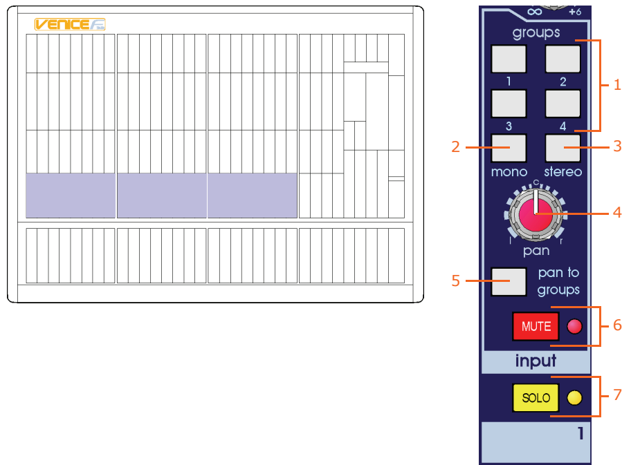
Groups and solo sections of the mono input channels
