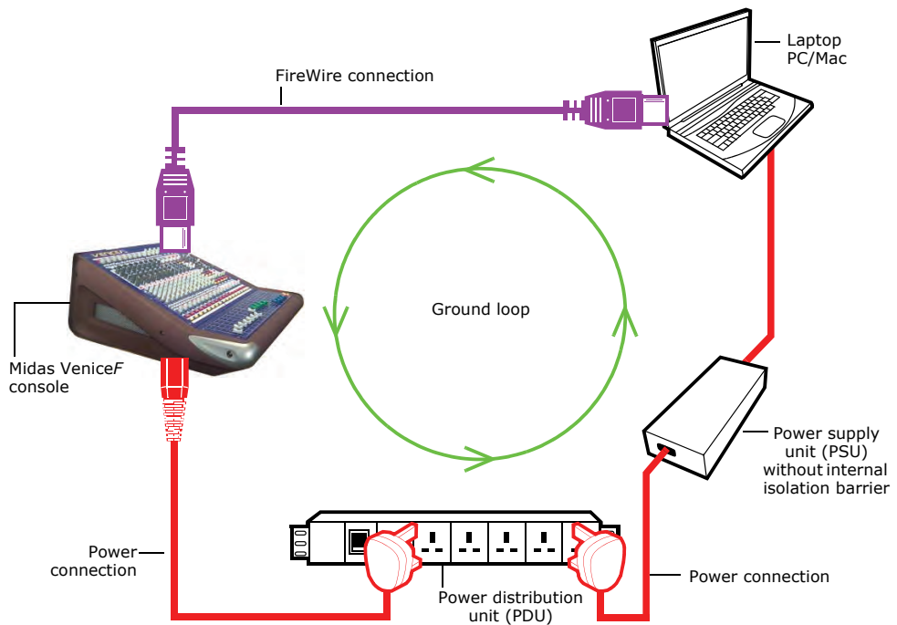
Non-isolated FireWire computer system. With no isolation barrier, the ground loop is present.
